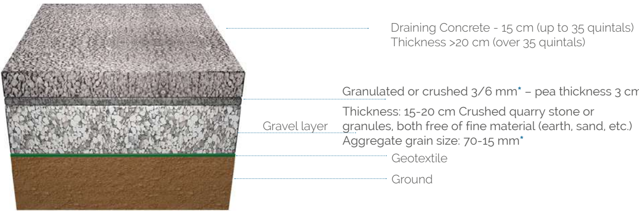
Prima Idro® permeable concrete - Version for traffic. * Nominal values
