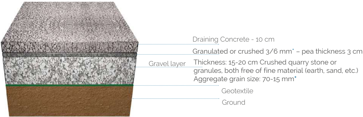
Prima Idro® permeable concrete - Pedestrian and cycle path * Nominal values
